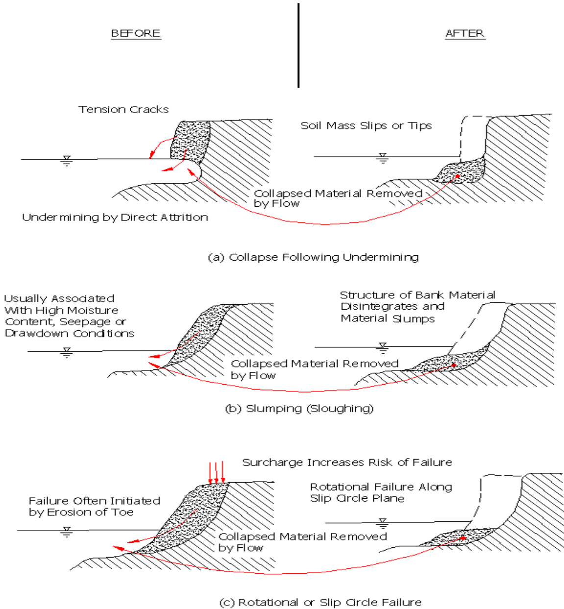
Figure 43.4 Mass Bank Failure Modes
