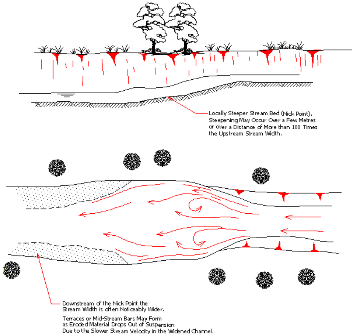
Figure 43.2 Typical Characteristics of Bed Scour
