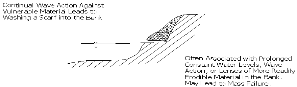
(b) Bank Undercutting
