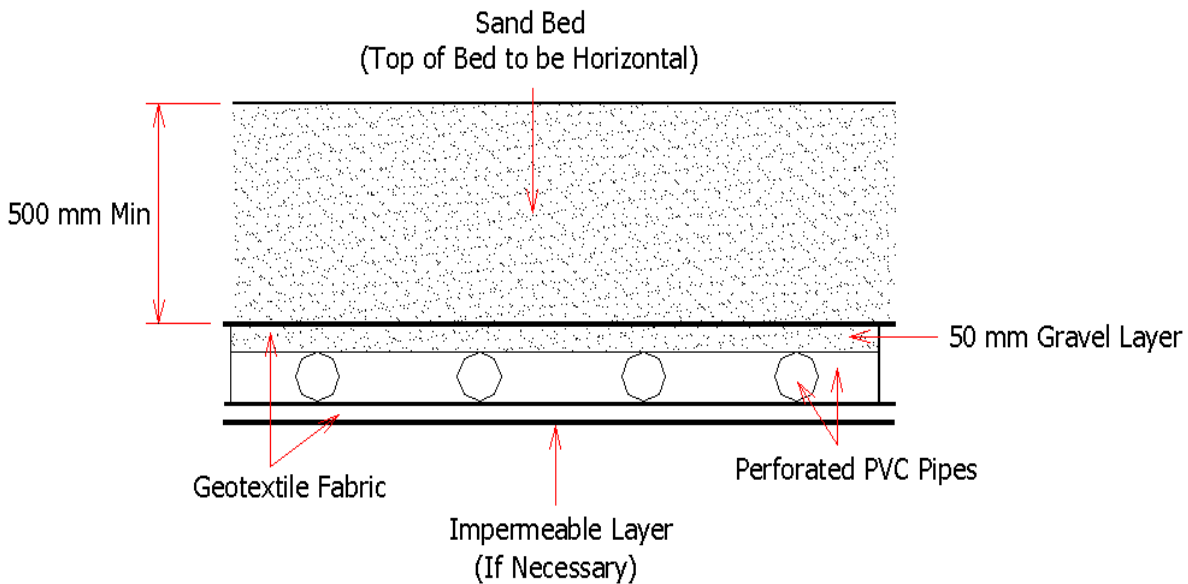
Figure 31.8 Sand Bed Profile with Gravel Layer
