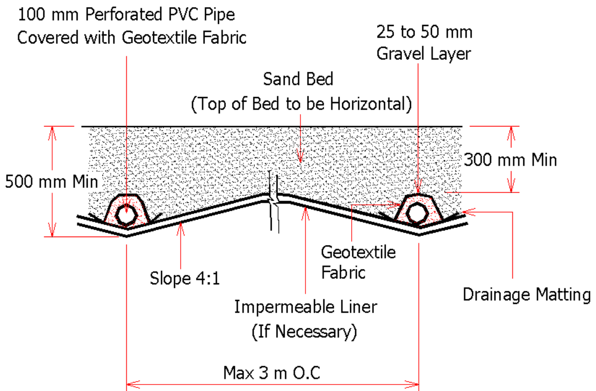
Figure 31.9 Sand Bed Profile with Trench Design (Source : City of Austin, 1988)
