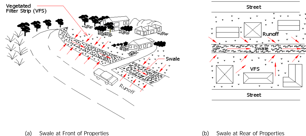
Figure 31.1 Typical Application of Swale and Vegetated Filter Strips
