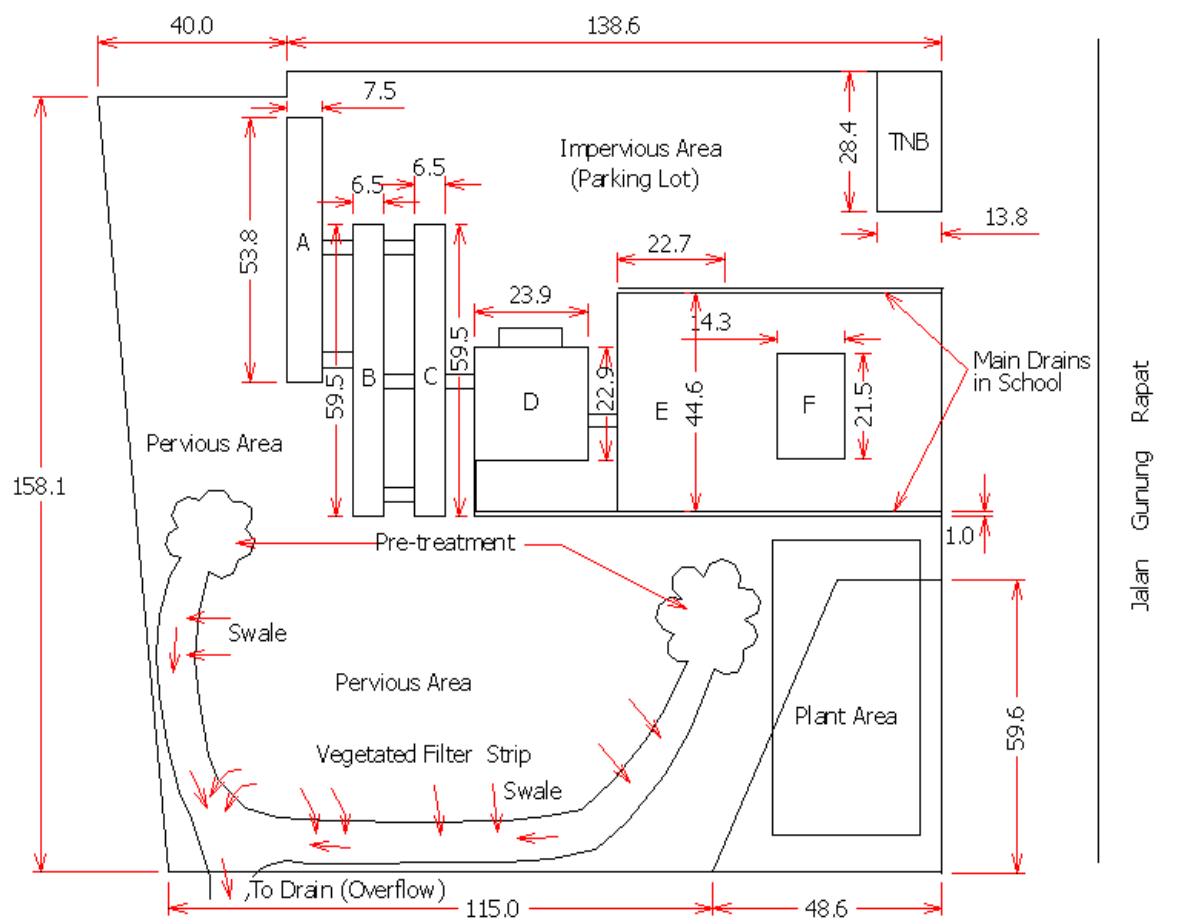
Figure 31.A1 Swale Layout for Sekolah Menengah Seri Ampang at Rapat Setia, Ipoh.
