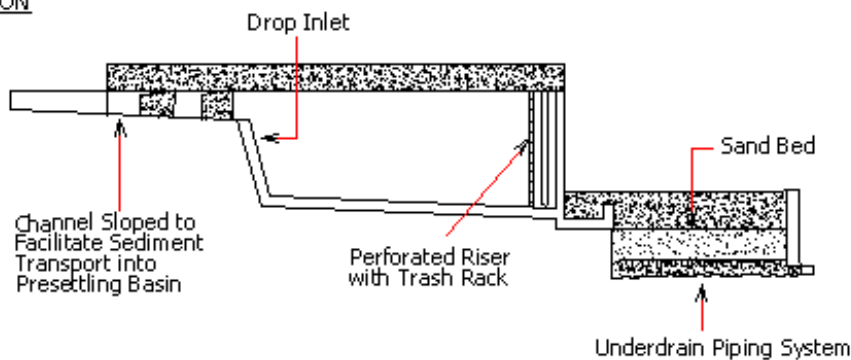
Figure 31.6 Sand Filtration Basin Preceded By Presettling Basin
