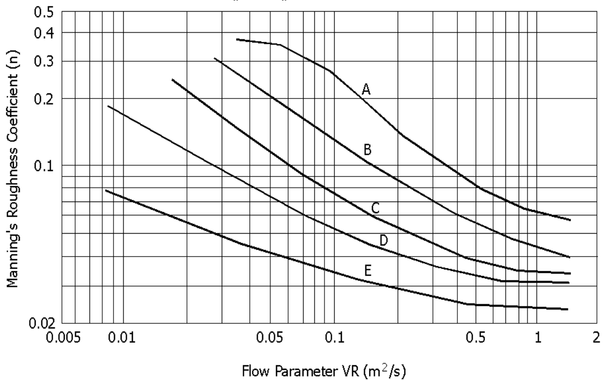
Figure 31.3 Resistance of Grasslined Channels. Curves are Given for 5 Resistance Classes, Determined from Table 31.2 (Source: U.S. Soil Conservation Service, 1985)
