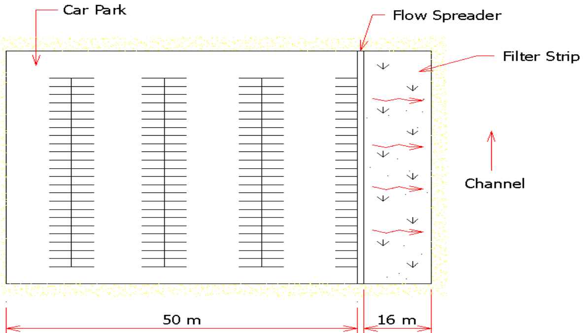
Figure 31.A3 Layout of Example Filter Strip
