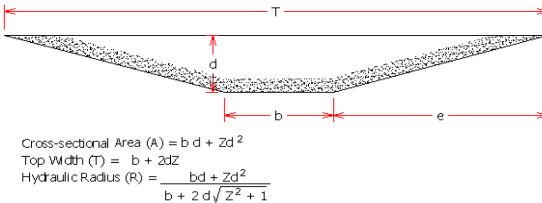
Figure 31.4 Cross-section and Hydraulic Radius for a Swale (U.S. Soil Conservation Service, as Reported in Department of Environmental Regulation, Florida, 1988).
