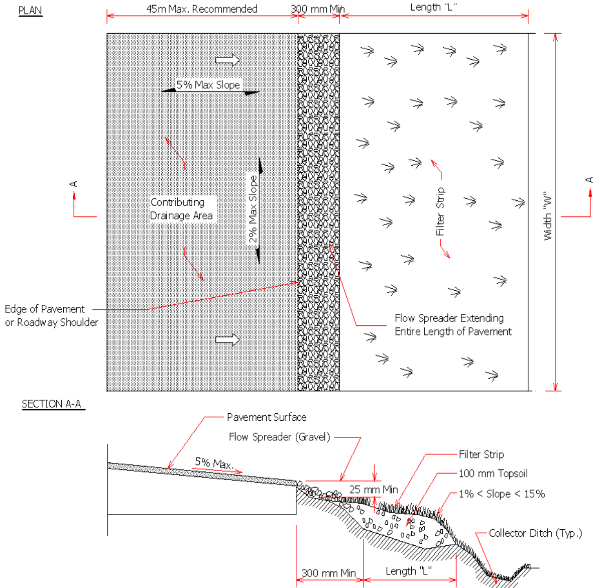
Figure 31.5 Plan and Cross Section of Typical Vegetated Filter Strip
