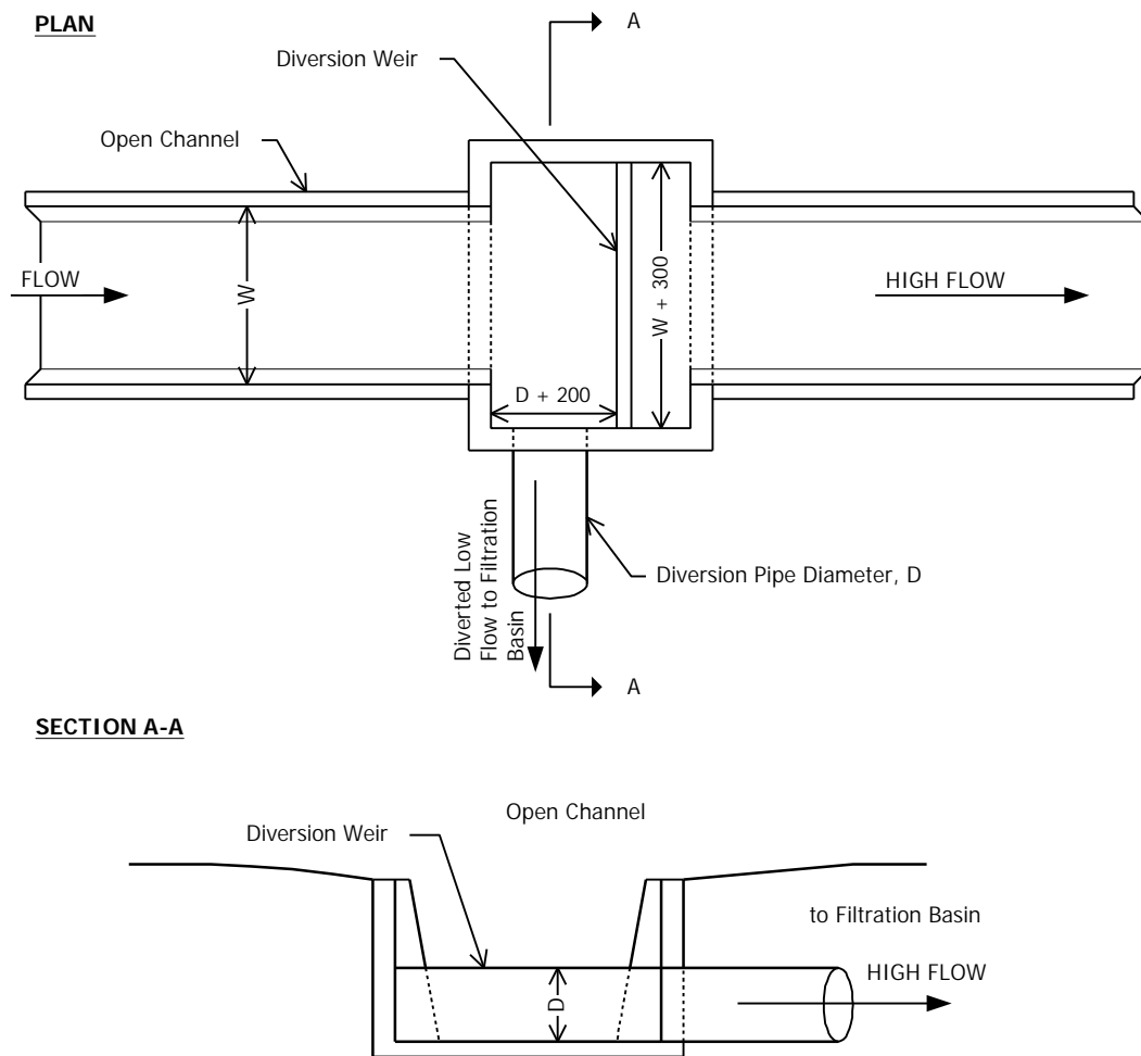
Figure 31.7 Typical Isolation/Diversion Structure
